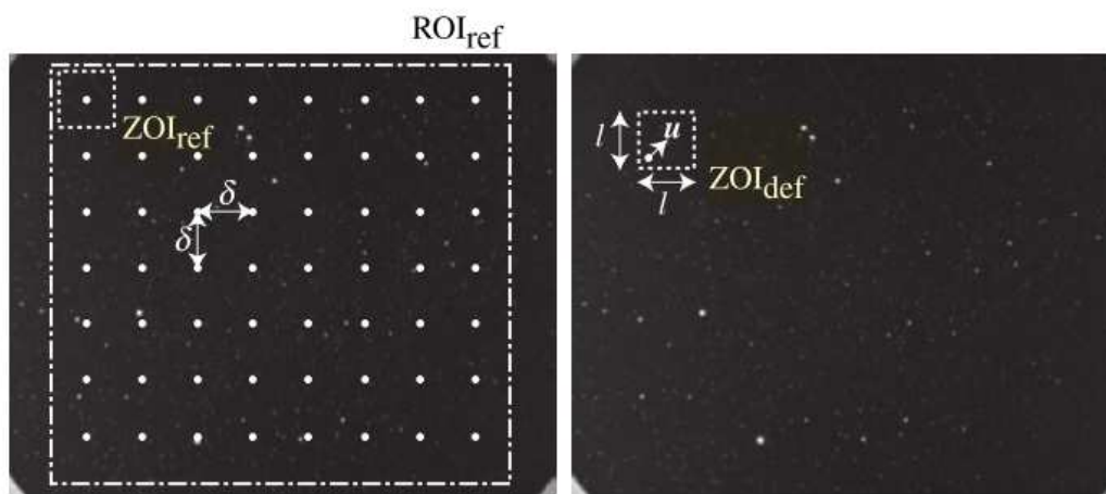
Figure 2. 50 - ROI and ZOI of a image (F. Hild &amp; Roux, 2006)
